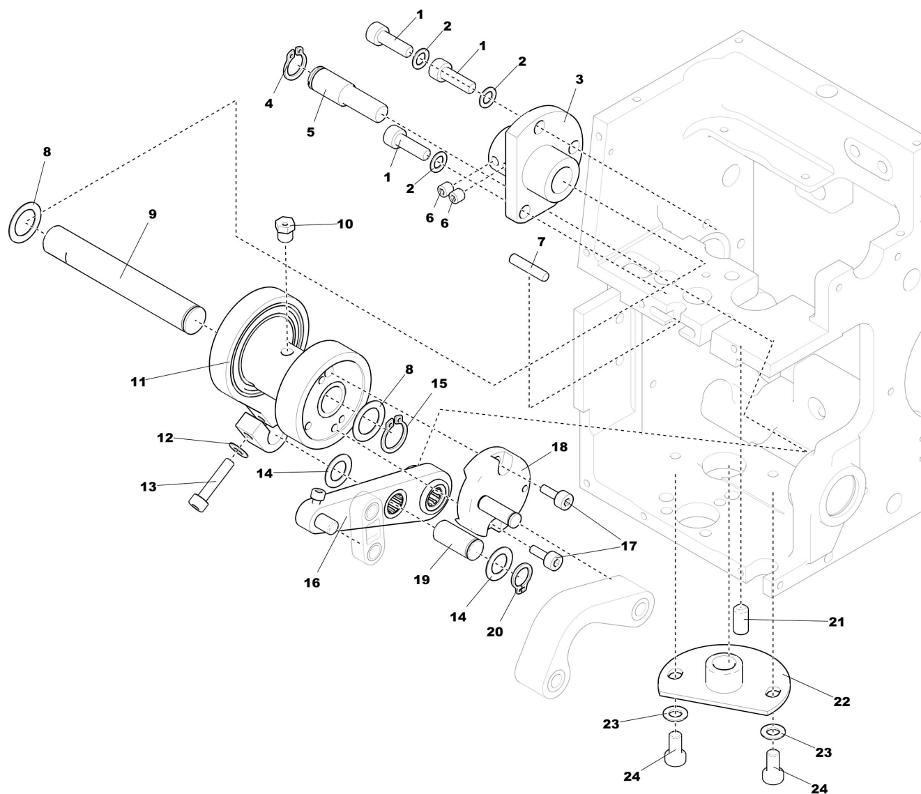
WKO-310 003 985 (B) - Antrieb (Nadelstange) / Drive (Needle Bar)
