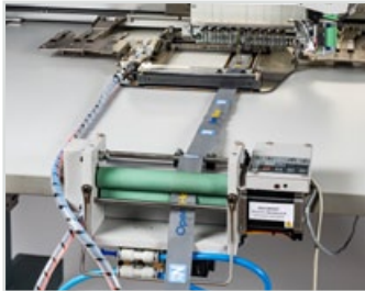
Fig 19 – ROLL2BASKET System
