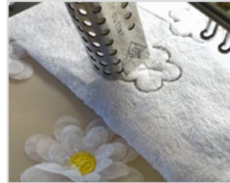
Fig 21 – Hot Air Cutting Device
